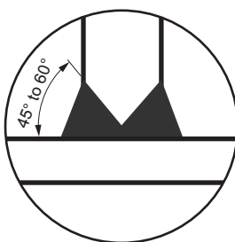
Figure 2 : k-type weld
