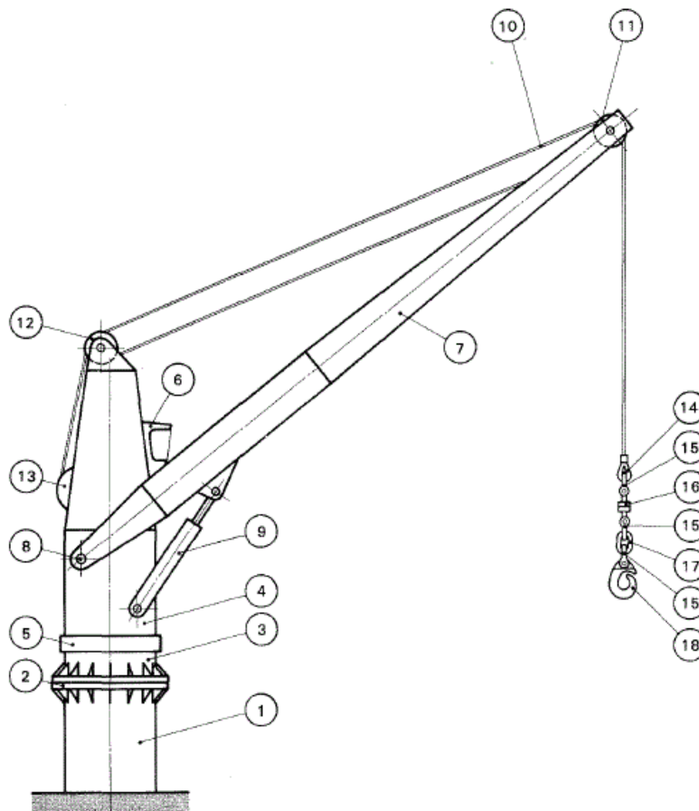
Figure 1 : Deck crane
