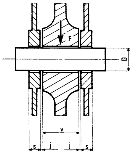
Figure 5 : Axle pin
