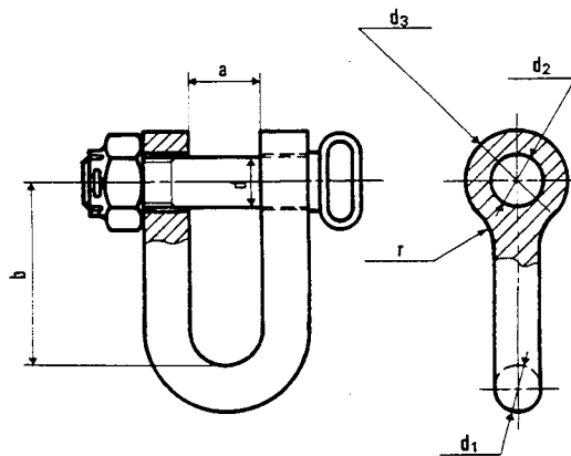
Figure 8 : Straight shackle
