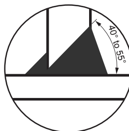
Figure 3 : V-type weld
