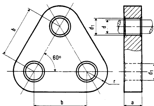
Figure 10 : Triangle plate
