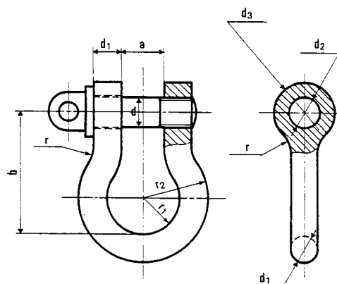
Figure 9 : Bow shackle
