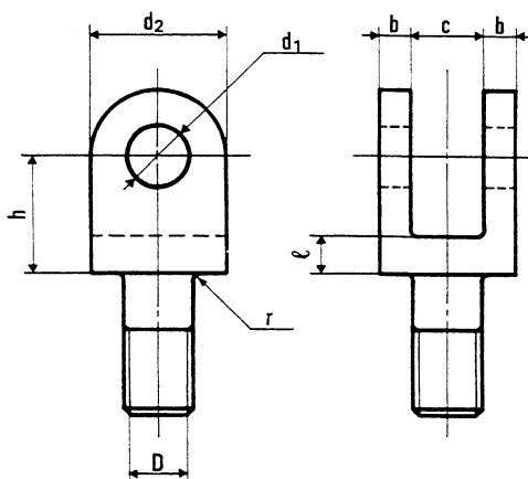
Figure 9 : Double lugs
