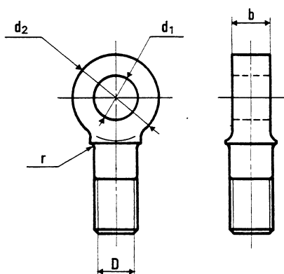
Figure 8 : Round eye
