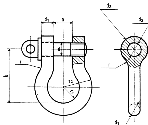
Figure 12 : Bow shackle
