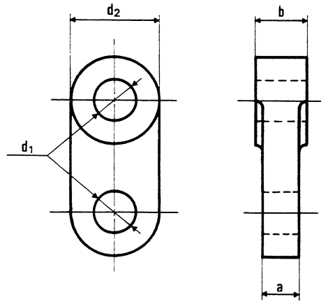
Figure 10 : Becket
