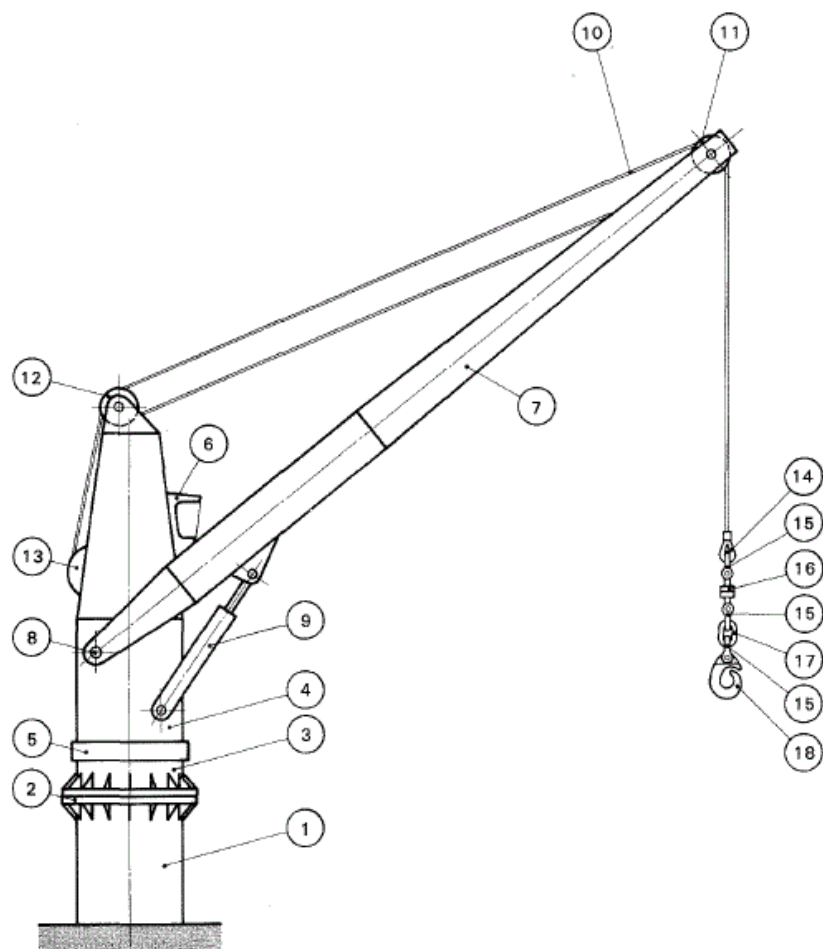
Figure 1 : Deck crane
