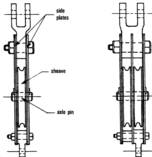
Figure 4 : Blocks
