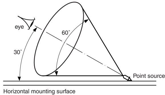
Figure 1 : Minimum luminance for LLL point sources mounted on horizontal surfaces
