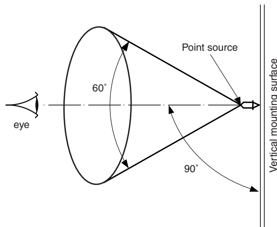
Figure 2 : Minimum luminance for LLL point sources mounted on vertical surfaces
