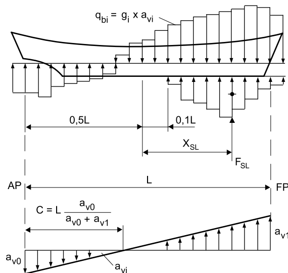
Figure 3 : Load due to impact on fore body
