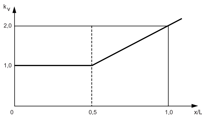
Figure 1 : k_v factor
