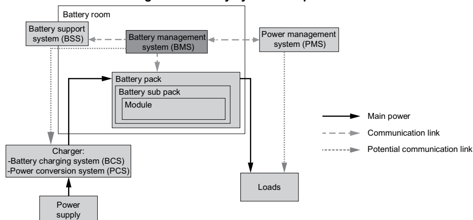
Figure 1 : Battery system components
