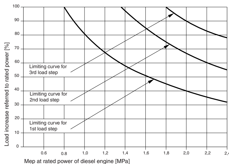
Figure 1 : Reference values for maximum possible sudden power increases P as a function of brake mean effective pressure, P_{me} , at declared power (four-stroke diesel engines)
