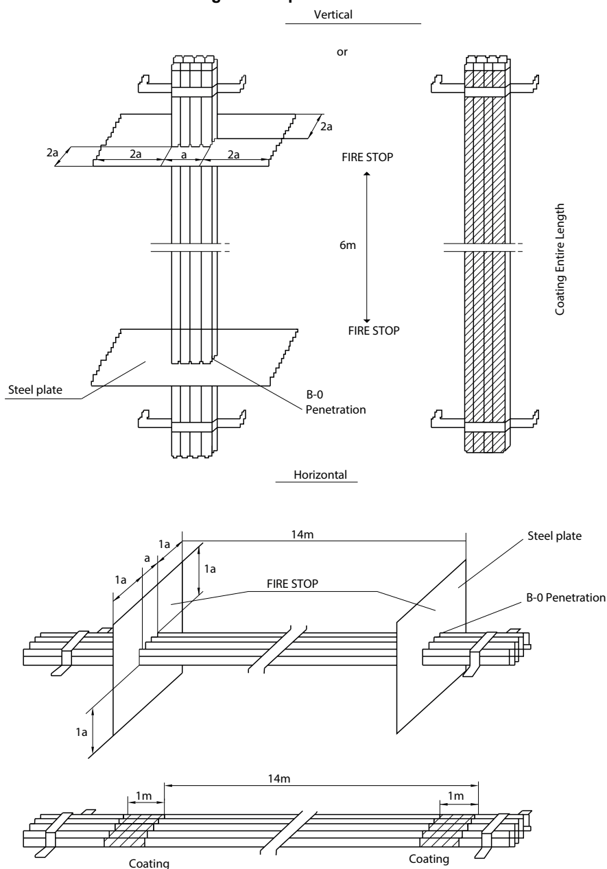
Figure 4 : Open cables runs
