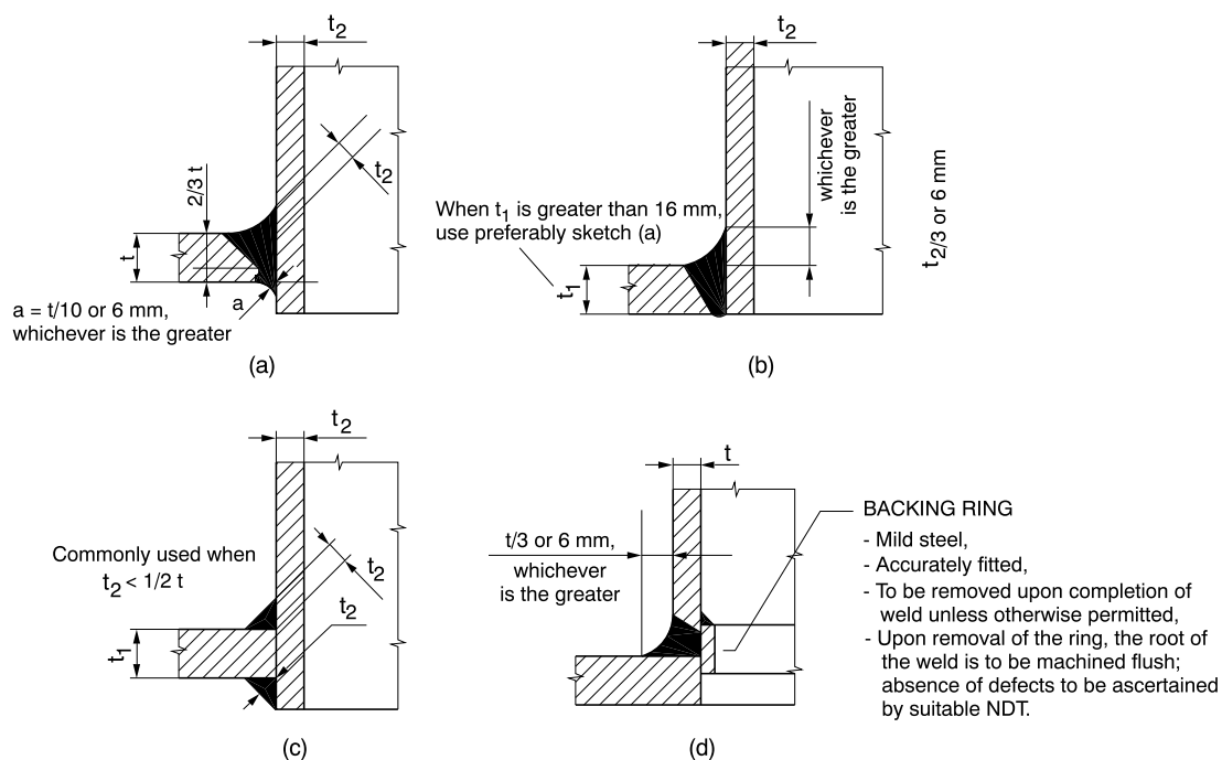
Figure 31 : Types of joints for nozzles and reinforcing rings (2)
