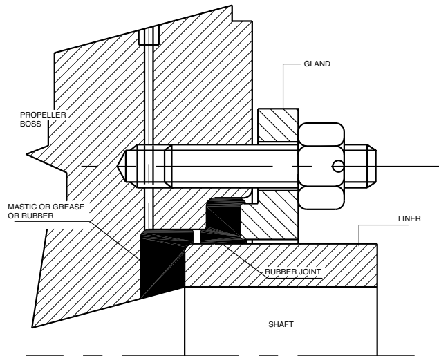
Figure 2 : Example of sealing arrangement
