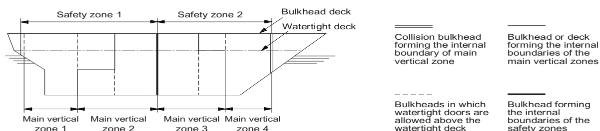
Figure 1 : Sample arrangement of main vertical zones and safety zones
