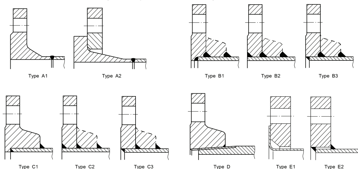
Figure 1 : Types of metallic flange connections
