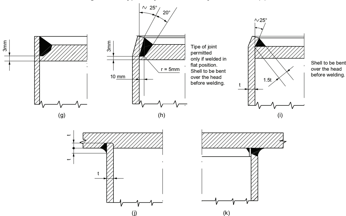
Figure 29 : Types of joints for unstayed flat heads (2)
