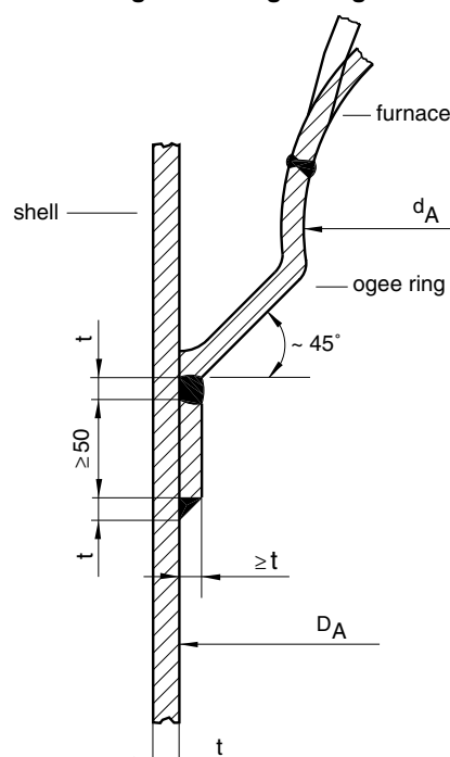
Figure 22 : Ogee ring
