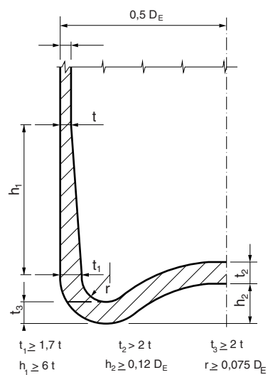
Figure 24 : Dished concave ends
