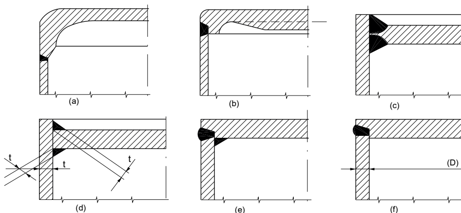
Figure 28 : Types of joints for unstayed flat heads (1)
