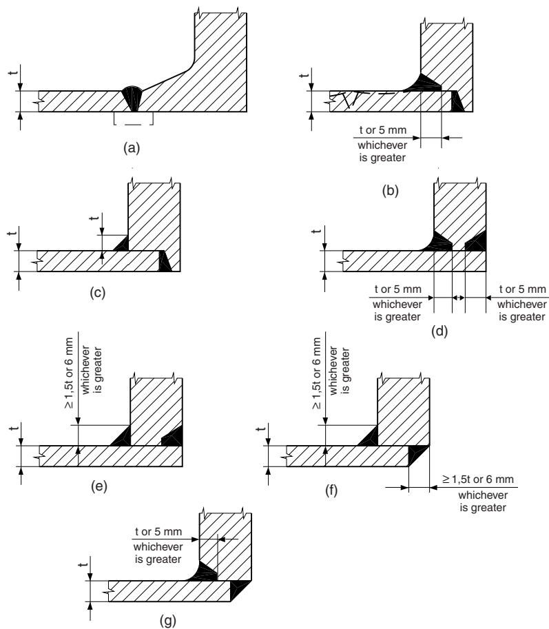
Figure 34 : Types of joints for flanges to nozzles
