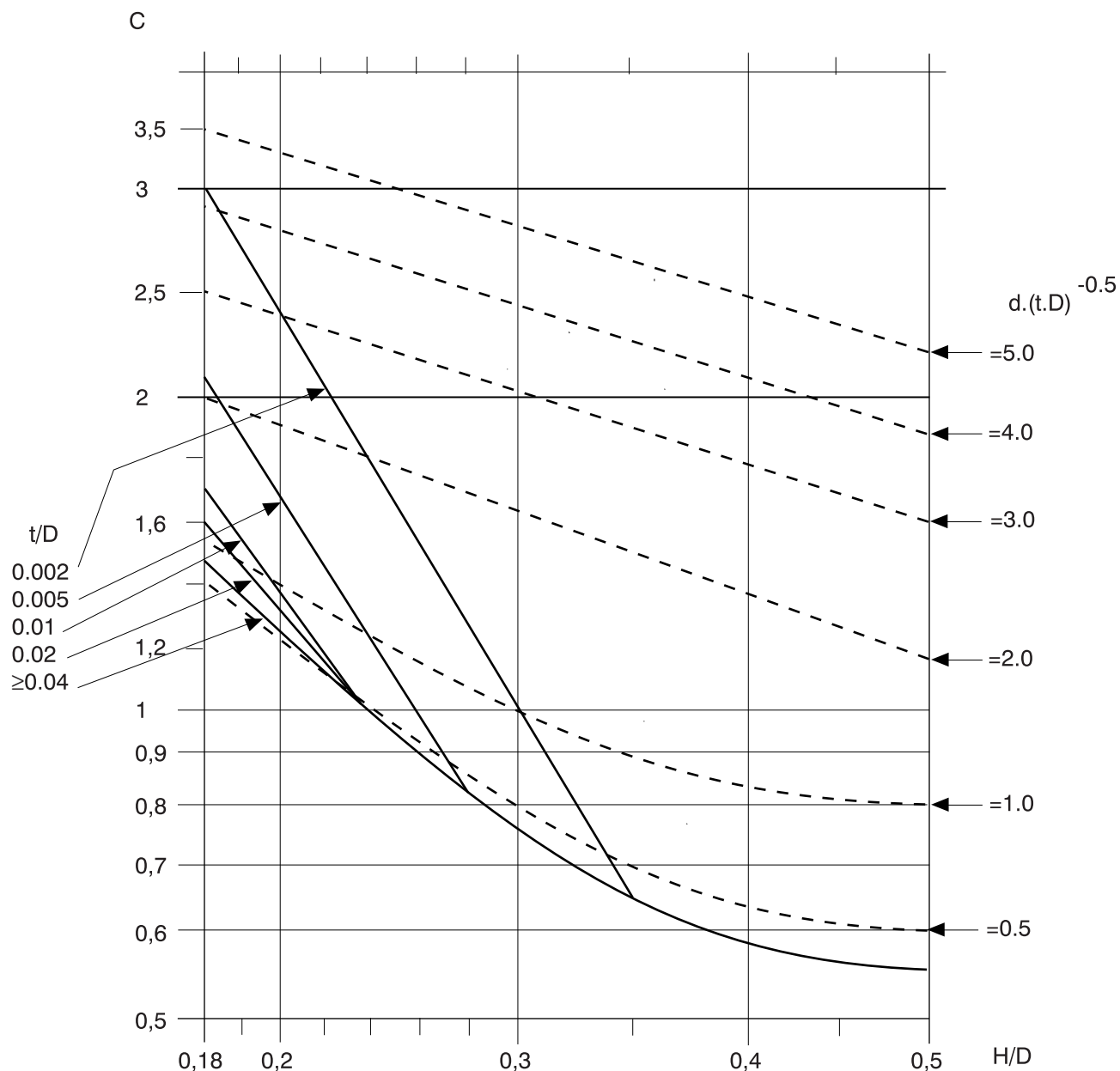
Figure 4 : Composed torispherical head
