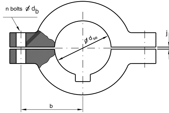
Figure 2 : Bolted tillers
