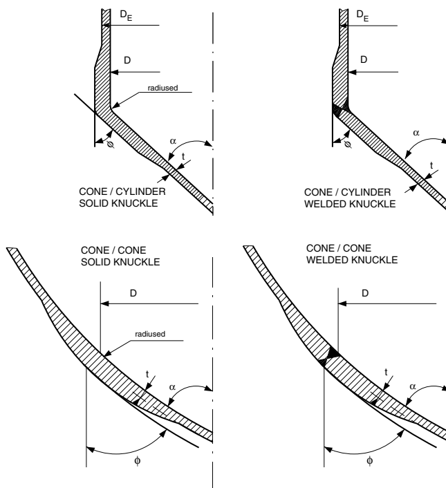
Figure 1 : Conic shells
