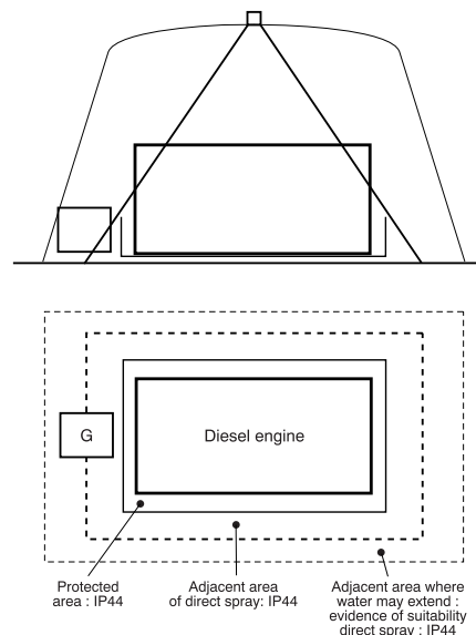
Figure 2 : Definitions of areas
