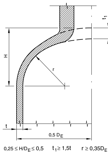
Figure 25 : Heads with openings
