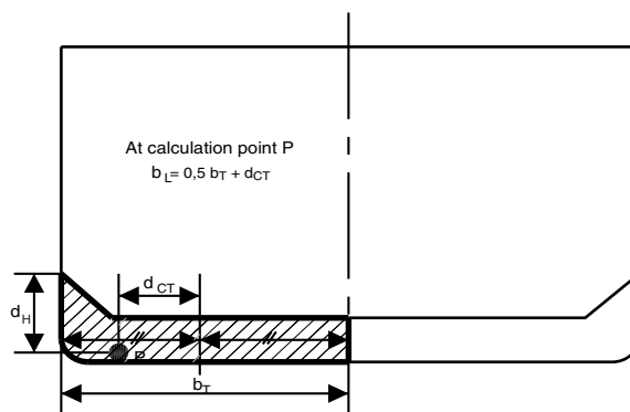
Figure 3 : Distances b_L and d_H
