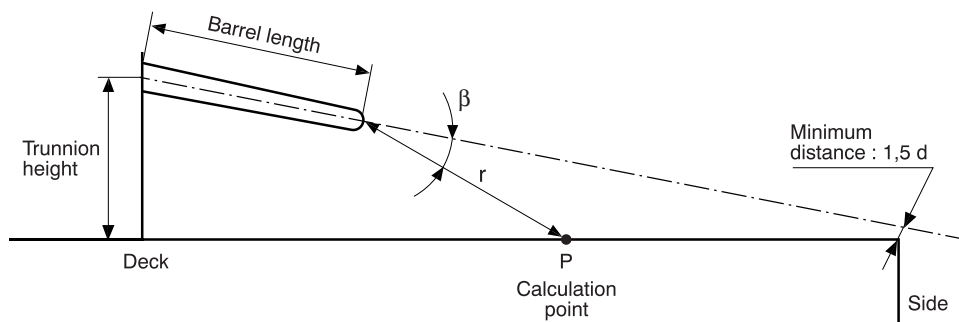
Figure 4 : Angle β and distance r for gun blast dynamic pressure calculation
