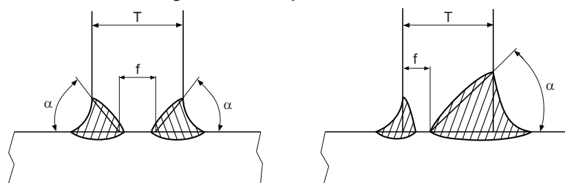
Figure 4 : Partial penetration weld
