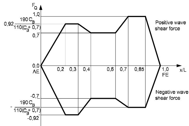
Figure 6 : Distribution factor F_Q
