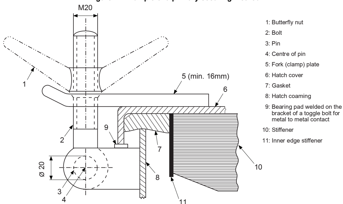
Figure 2 : Example of a primary securing method
