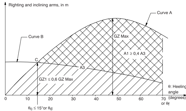
Figure 10 : Heavy cargo lifting criteria
