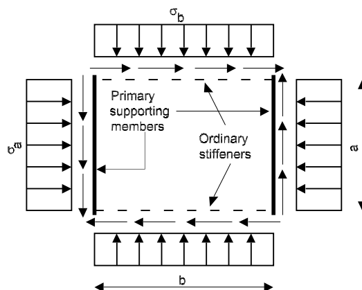
Figure 4 : Buckling of a simply supported rectangular plate panel subjected to bi-axial compression and shear
