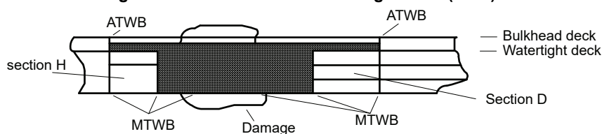
Figure 3 : Functions of the watertight deck (W.D.)
