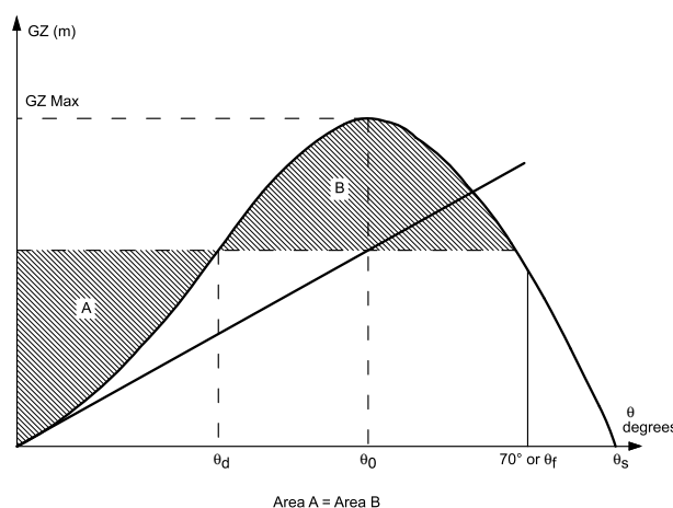
Figure 1 : Righting arms curve and angles
