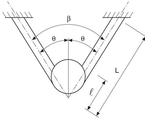
Figure 2 : Tangential type double arm bracket
