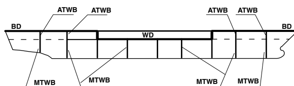
Figure 1 : Deck to which the margin line may be referred
