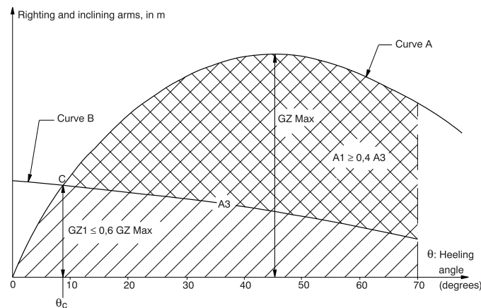
Figure 8 : High speed turning criteria
