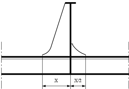
Figure 5 : End connection of ordinary stiffener - Backing bracket
