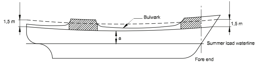
Figure 1 : Ships with perpendicular front bulkhead Effective area of bulwarks or fixed screen to be included in the equipment number
