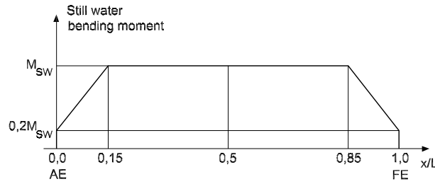
Figure 2 : Preliminary still water bending moment distribution
