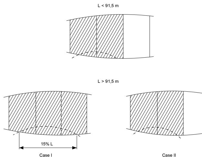
Figure 1 : Standard damage case - Longitudinal extension (example of damage on the shell and extension of flooding)
