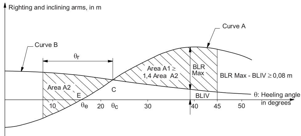
Figure 4 : Righting arms curve and heeling arms caused by severe wind and rolling
