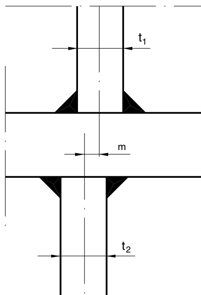
Figure 9 : Misalignment in cruciform connections
