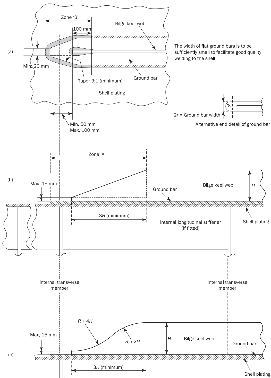
Figure 3 : Single web bilge keel design
