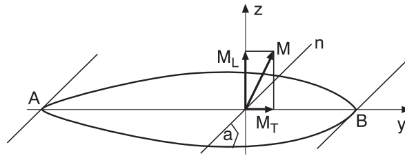
Figure 3 : Locations of maximum stress under combined bending
