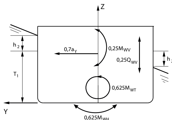
Figure 3 : Wave loads in load case "c"
