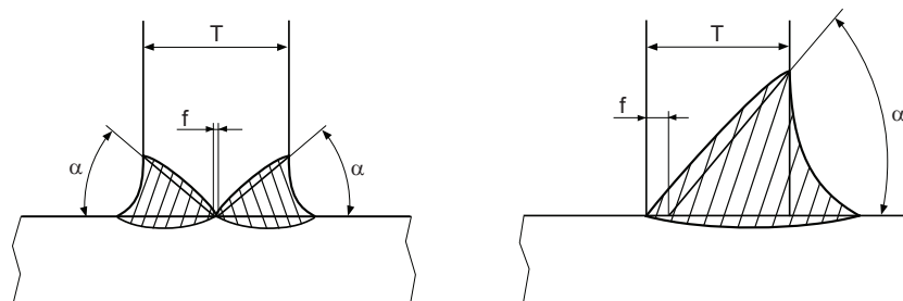
Figure 5 : Full penetration weld
