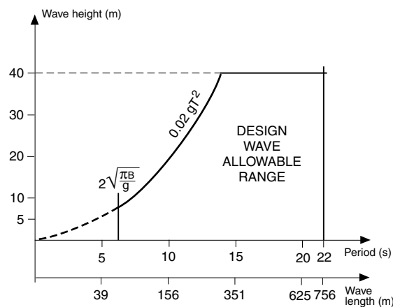
Figure 2 : Allowable range of design waves
