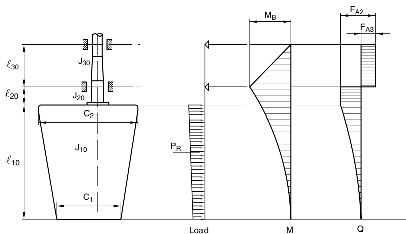
Figure 2 : 2 bearing rudders with solepiece
