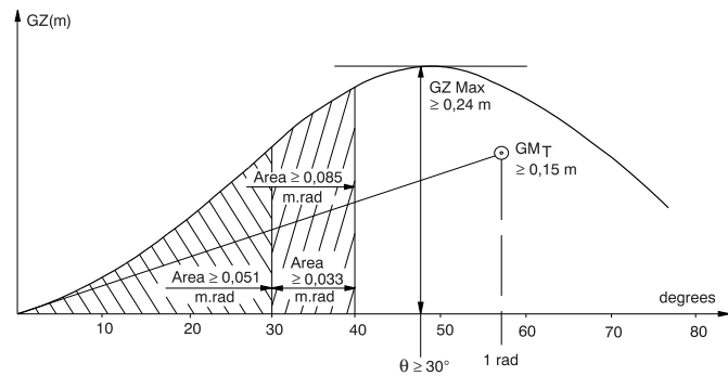
Figure 6 : Icing criteria without wind
