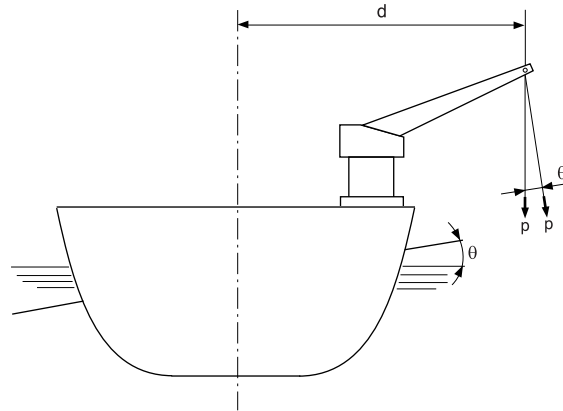
Figure 9 : Heavy cargo lifting
