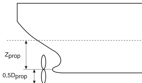
Figure 1 : Dimensions for calculation of relative motion Z_{PE}
