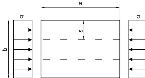
Figure 2 : Buckling of stiffeners parallel to the direction of compression
