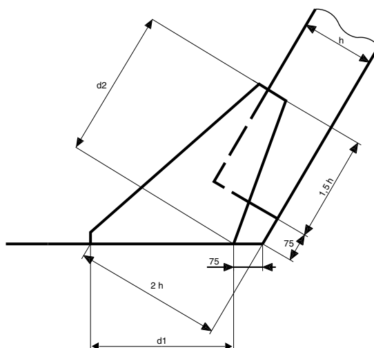
Figure 4 : Lower brackets of main frames
