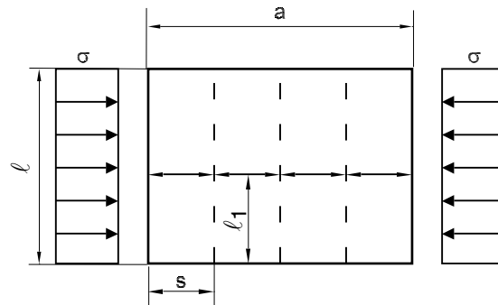
Figure 4 : Buckling of stiffeners perpendicular to the direction of compression (intercostal stiffeners)
