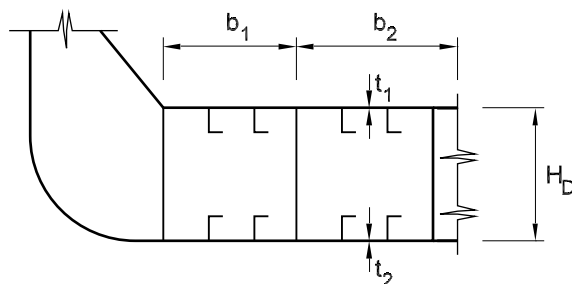
Figure 4 : Beams of double skin structures
