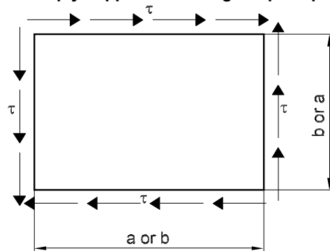
Figure 3 : Buckling of a simply supported rectangular plate panel subjected to shear
