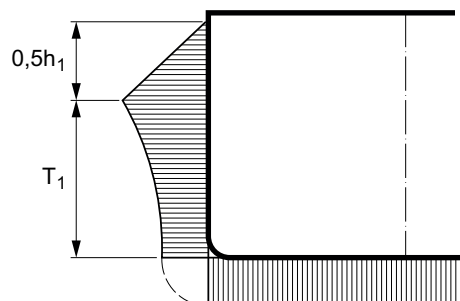
Figure 3 : Wave pressure in load case “b”
