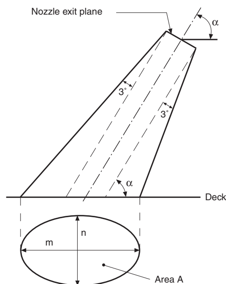
Figure 3 : Missile blast impingement area
