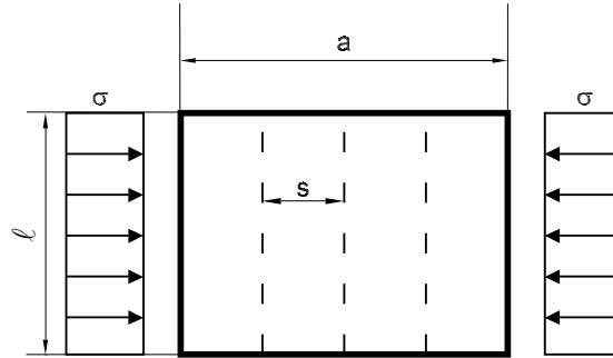
Figure 3 : Buckling of stiffeners perpendicular to the direction of compression
