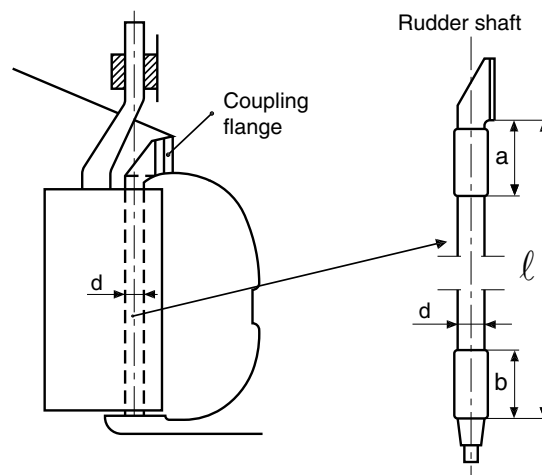
Figure 12 : Simplex rudder shaft geometry
