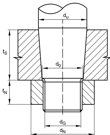
Figure 5 : Geometry of cone coupling
