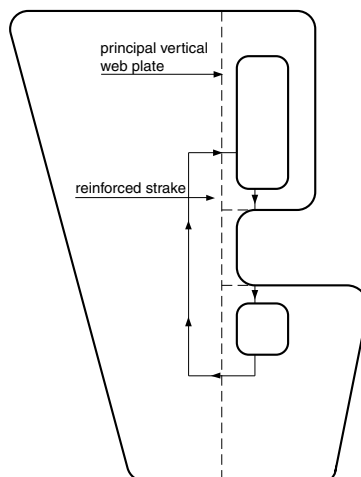
Figure 6 : Reinforced strake extension for semi-spade rudders
