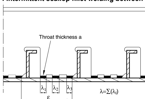
Figure 2 : Intermittent scallop fillet welding between cut-outs
