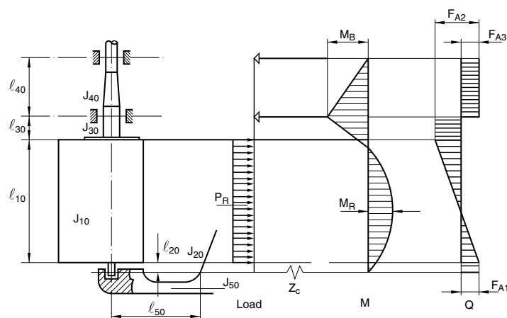
Figure 2 : 2 bearing rudders with solepiece
