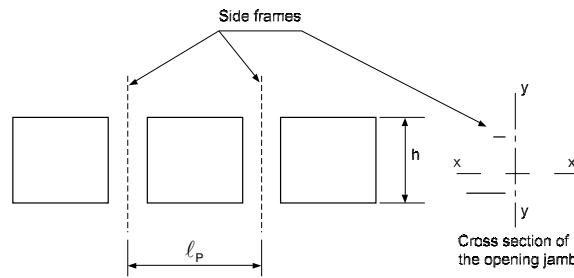
Figure 3 : Side openings
