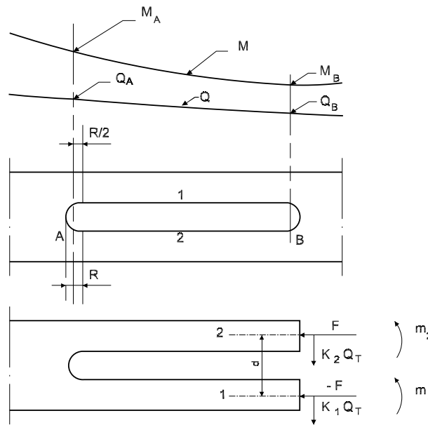
Figure 8 : Large openings in primary supporting members - Secondary stresses
