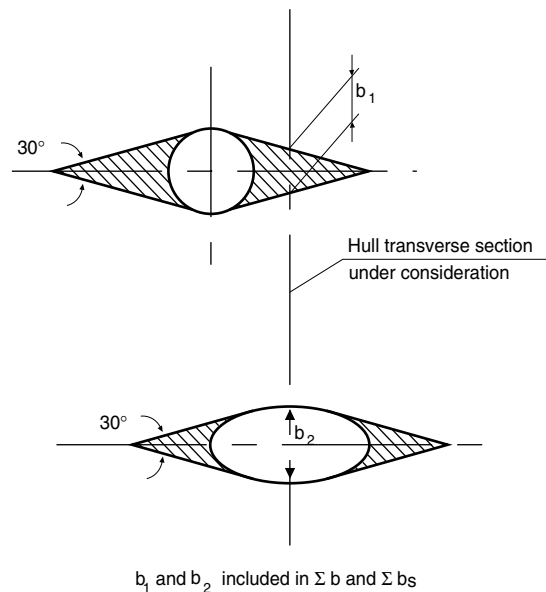
Figure 2 : Calculation of \Sigma b and \Sigma b_s
