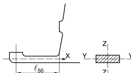
Figure 4 : Solepiece geometry
