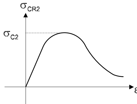
Figure 5 : Load-end shortening curve \sigma_{CR2}-\epsilon for flexural-torsional buckling
