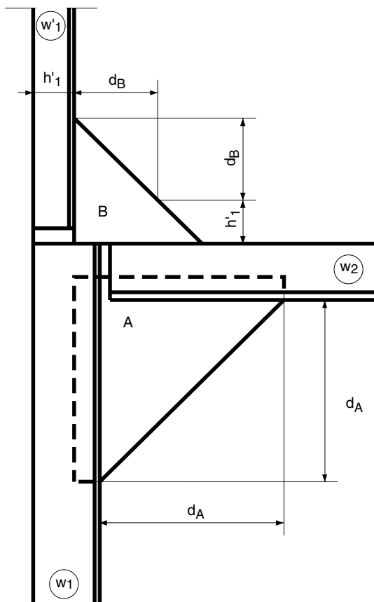
Figure 3 : Connections of frames to deck beams
