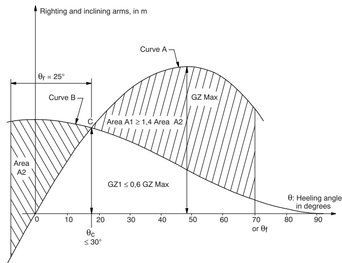
Figure 5 : Severe wind and rolling criteria
