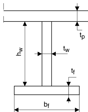
Figure 3 : Dimensions of a built section
