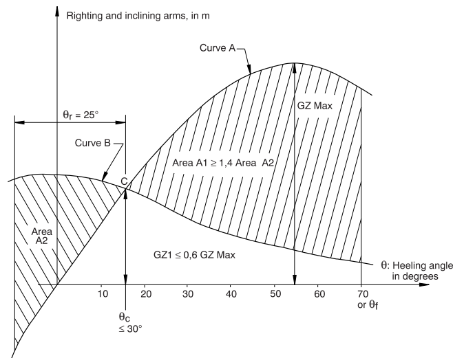
Figure 7 : Icing criteria with wind
