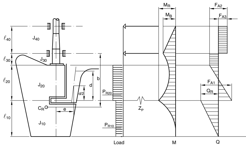
Figure 3 : 2 bearing semi-spade rudders with rudder horn
