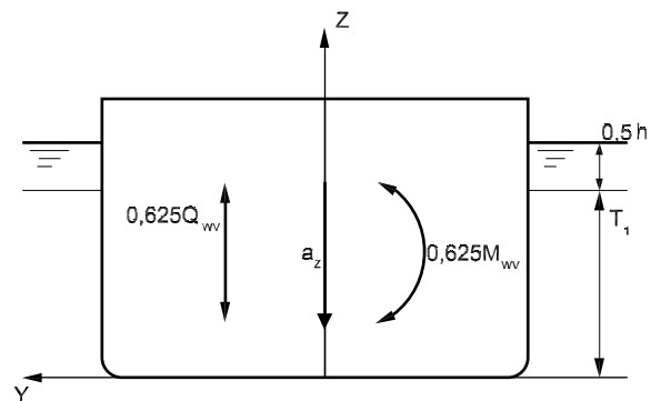
Figure 2 : Wave loads in load case “b”
