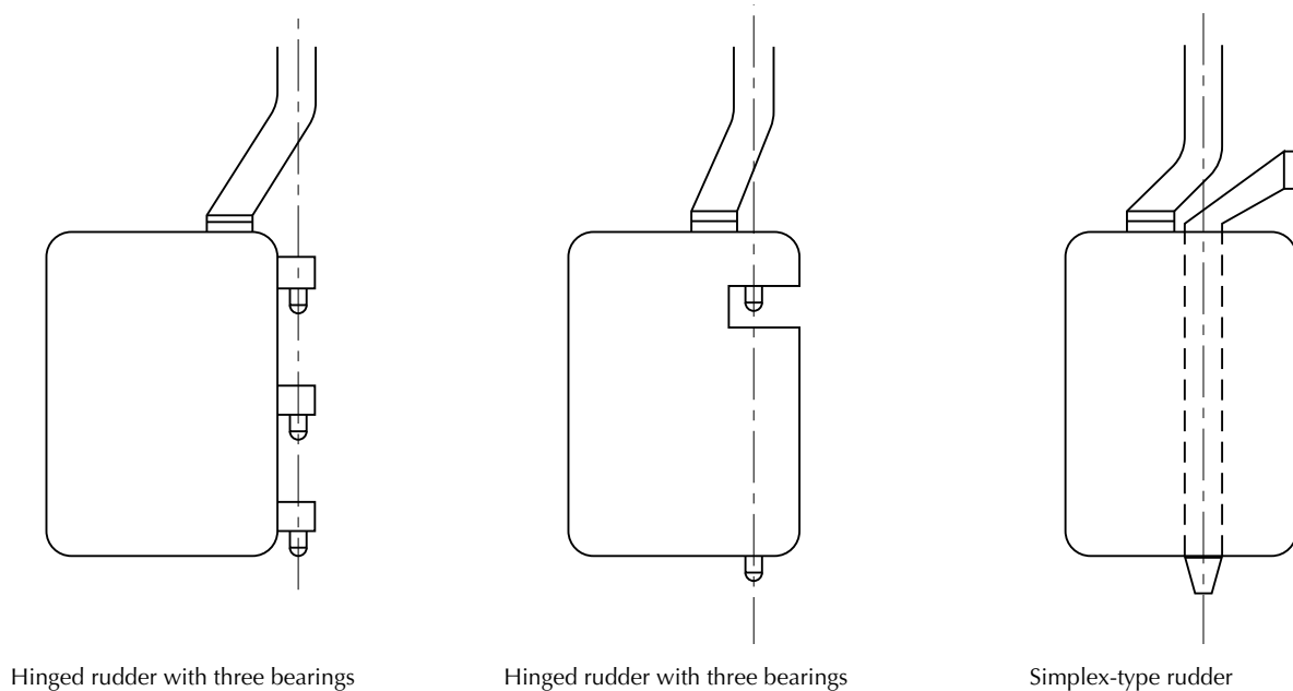
Figure 4 : Rudder types
