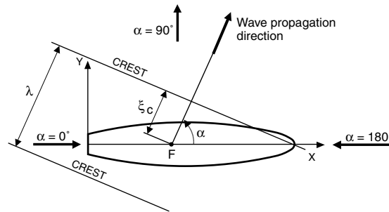
Figure 1 : Wave heading
