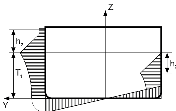
Figure 4 : Wave pressure in load case “c”
