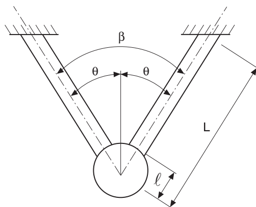
Figure 1 : Radial type double arm bracket
