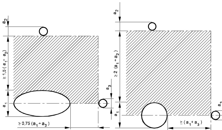
Figure 2 : Circular openings in the strength deck
