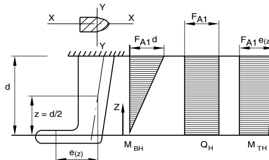
Figure 10 : Rudder horn geometry
