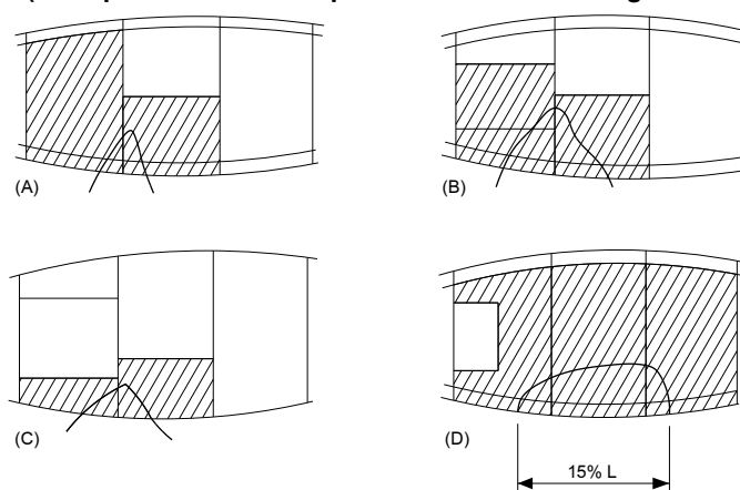
Figure 3 : Standard damage case - Transversal extension (example of transversal penetration and flooding extension)
