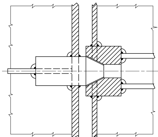
Figure 3 : Thrust bearing
