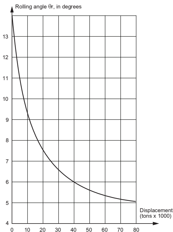
Figure 1 : Rolling angles to be taken into account in damage stability calculations, valid also in “V” Line tracing
