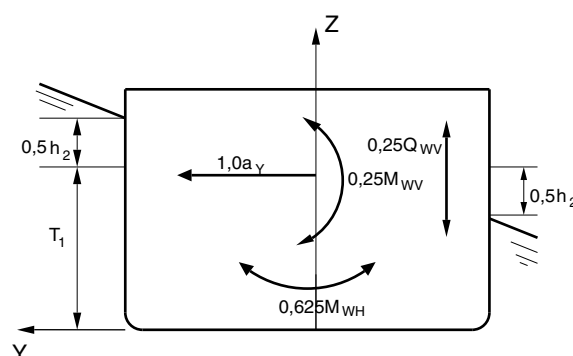
Figure 4 : Wave loads in load case "d"
