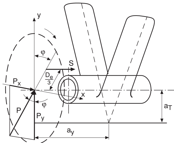
Figure 4 : Definition of forces, directions and distances
