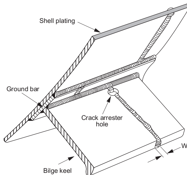
Figure 2 : Single web bilge keel arrangement
