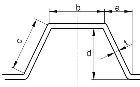
Figure 3 : Corrugated bulkhead
