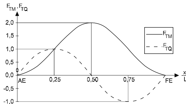
Figure 4 : Ship condition 1 - Distribution factors F_{TM} and F_{TQ}
