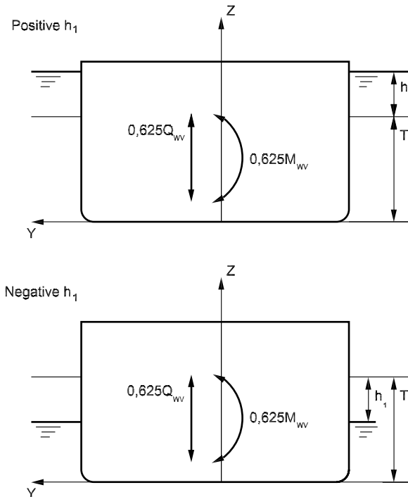
Figure 1 : Wave loads in load case “a”
