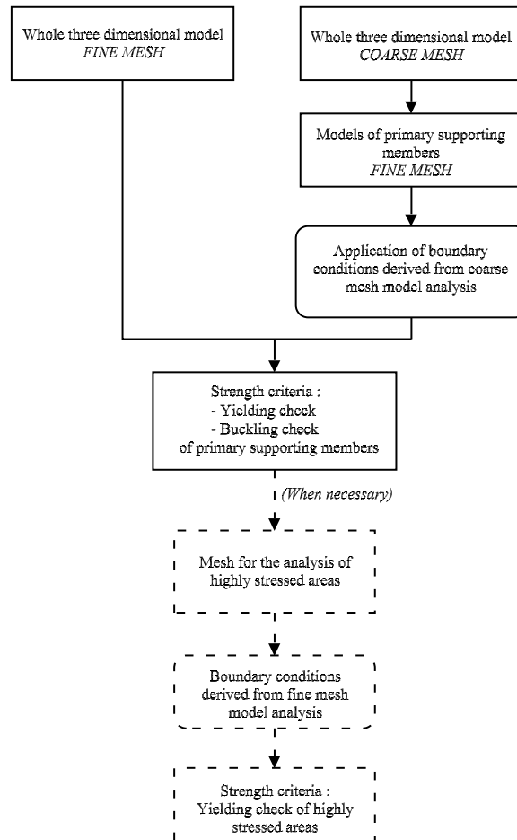
Figure 2 : Finite element modelling criteria
