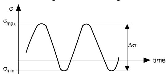
Figure 2 : Stress range
