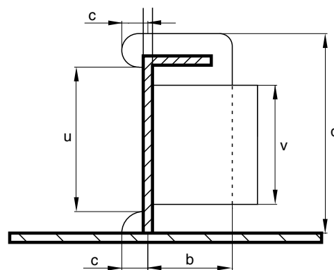
Figure 3 : End connection of ordinary stiffener - Dimensions of the cut-out
