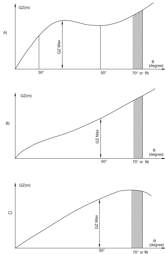
Figure 4 : GZ Max to be considered
