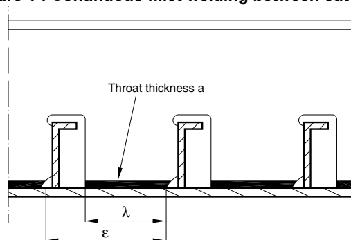
Figure 1 : Continuous fillet welding between cut-outs
