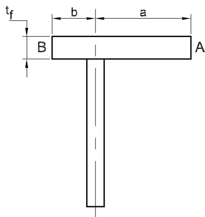
Figure 3 : Geometry of a stiffener section
