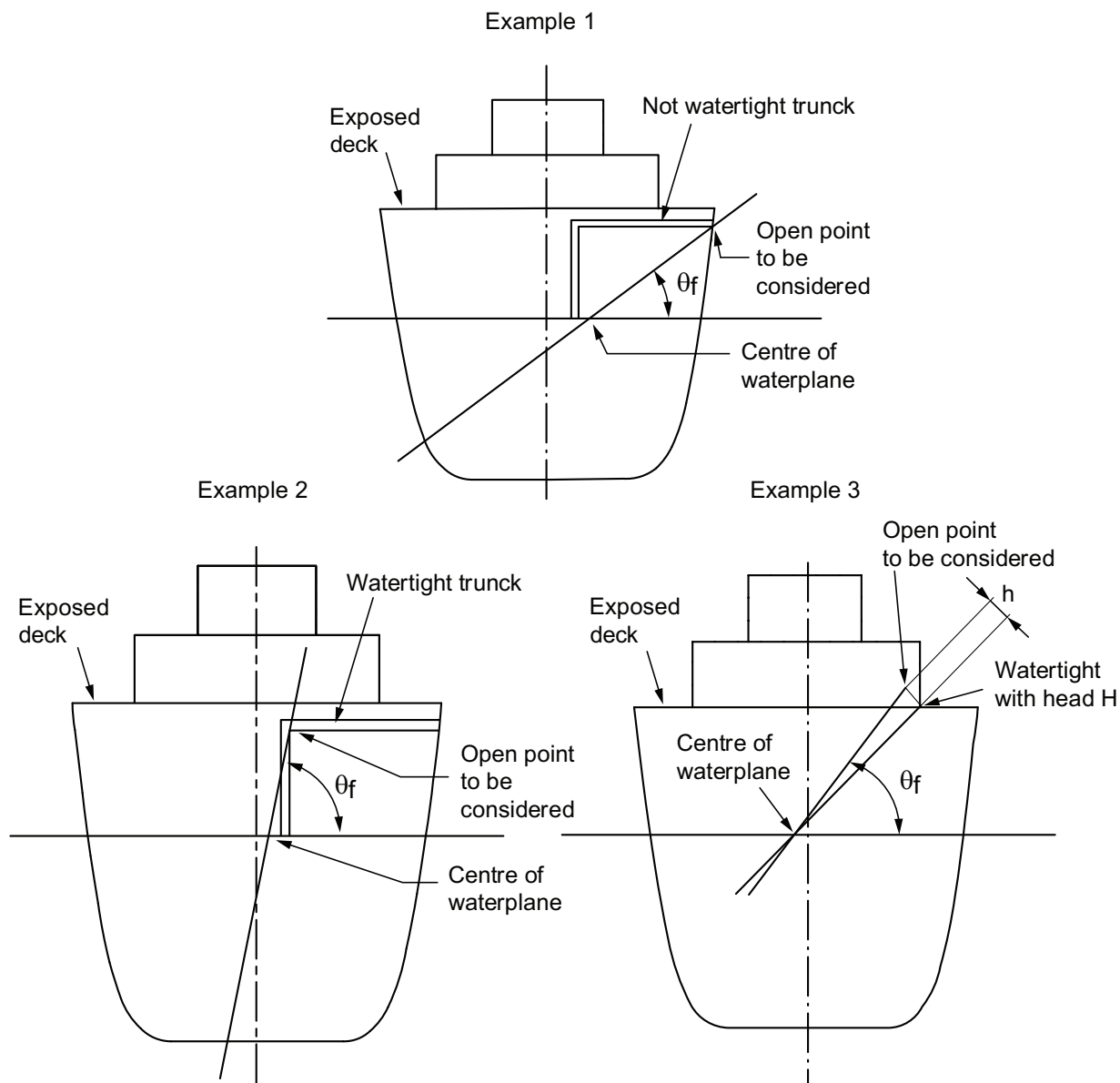
Figure 2 : Flooding angle - Example 1
