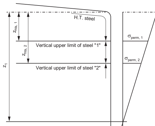
Figure 3 : Vertical extent of higher strength steel
