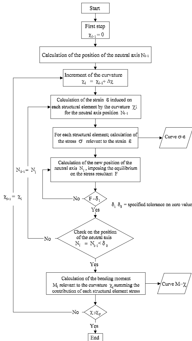
Figure 2 : Flow chart of the procedure for the evaluation of the curve M-\chi
