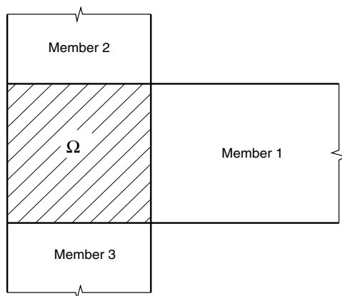
Figure 7 : Bracketless end connections of primary supporting members
