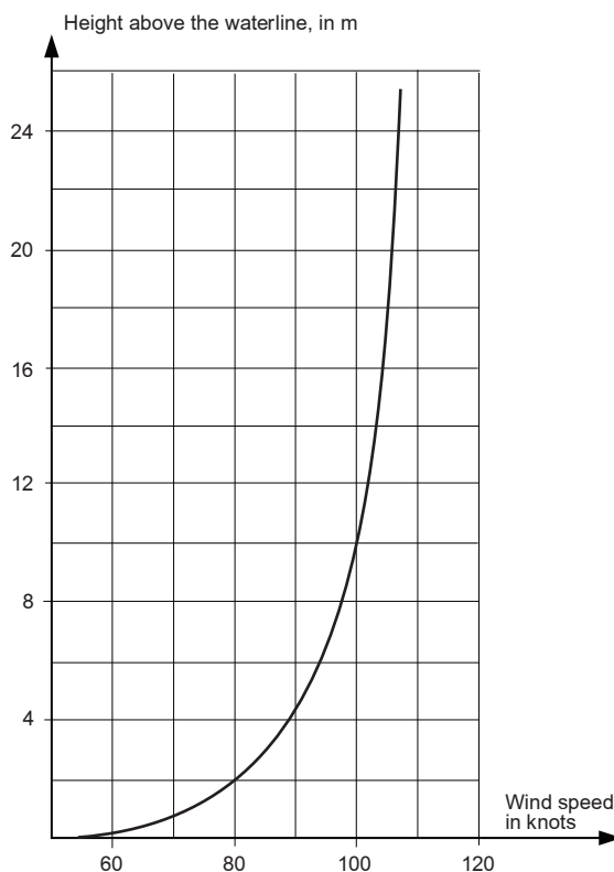
Figure 1 : Speed of the wind as a function of the height above the waterline
