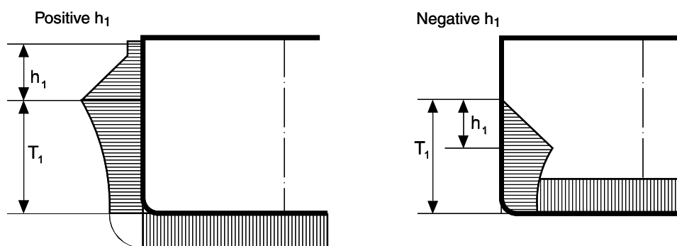
Figure 2 : Wave pressure in load case “a”
