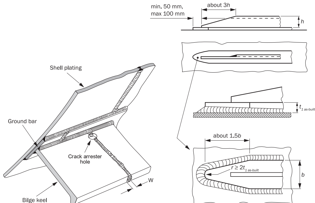
Figure 6 : Connections of single web bilge keels
