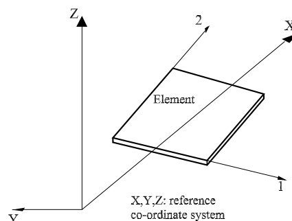
Figure 5 : Reference and element co-ordinate systems
