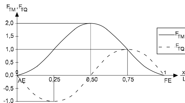
Figure 5 : Ship condition 2 - Distribution factors F_{TM} and F_{TQ}
