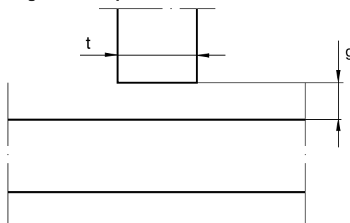
Figure 7 : Gap in fillet weld T connections
