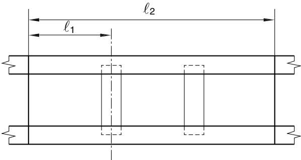
Figure 2 : Span of ordinary stiffeners in the case of open floors
