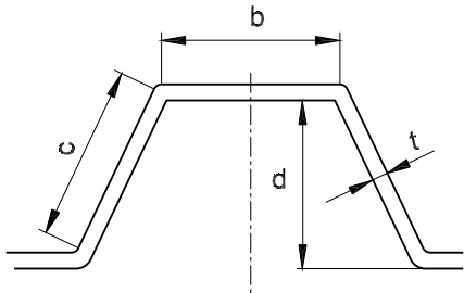
Figure 4 : Dimensions of a corrugation
