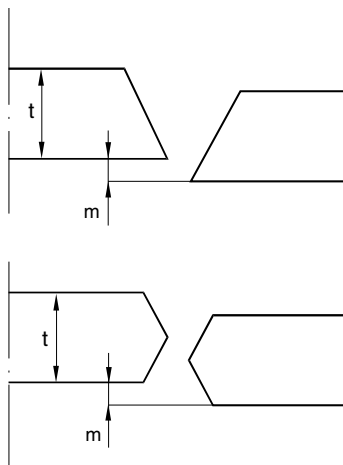
Figure 8 : Plate misalignment in butt connections
