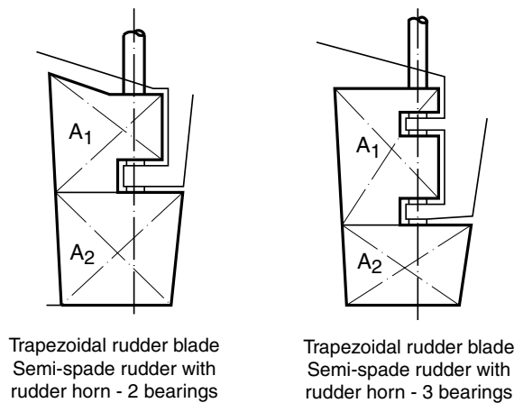
Figure 2 : Rudder blades with cut-outs
