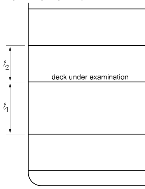
Figure 3 : 'Tweendeck heights for grillage analysis of deck primary supporting members
