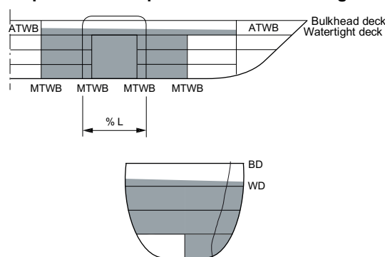
Figure 2 : Standard damage case - Vertical extension (example of vertical penetration and flooding extension)
