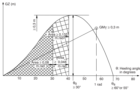
Figure 3 : Righting arms curve criteria
