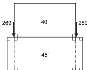
Figure 17 : Permissible vertical compression on frames of 40' containers supported by 45' containers
