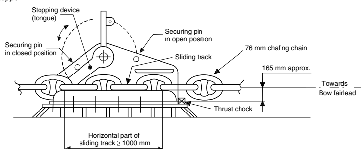
Bar hinged type chain stopper
