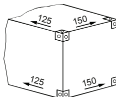
Figure 12 : Permissible transverse and vertical compressions on end frames of 20', 30' and 40' ISO containers
