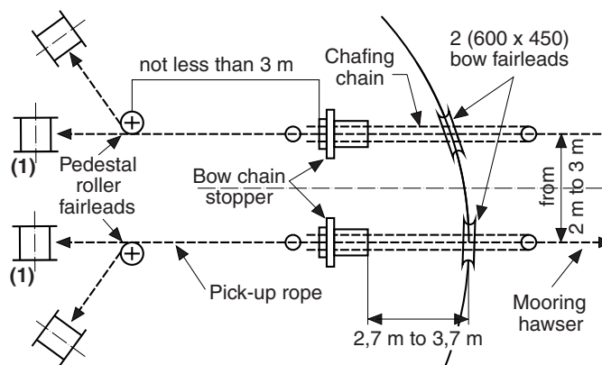
Figure 3 : Forecastle schematic layout for DWT > 150000 t
