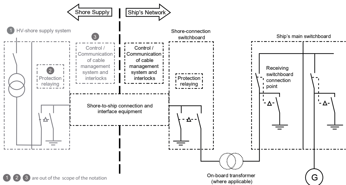
Figure 1 : Diagram of a typical OPS arrangement
