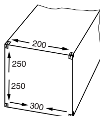
Figure 14 : Permissible transverse and vertical tensions on end frames of 20', 30', 40' and 45' ISO containers
