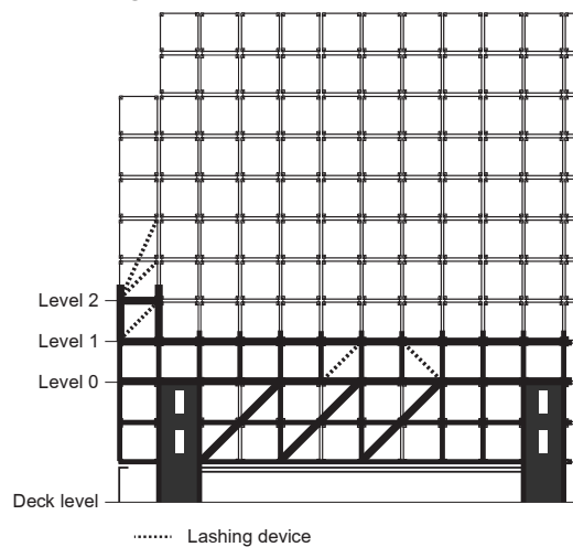
Figure 10 : Level of attachment
