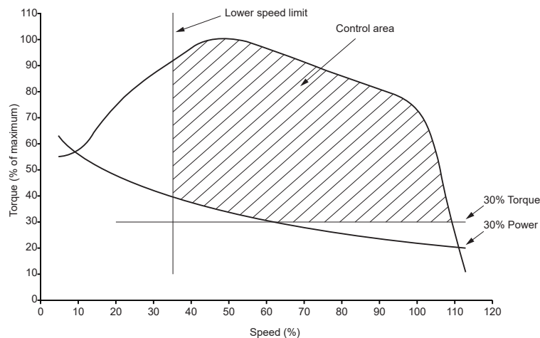
Figure 1 : Control area for variable speed auxiliary engines
