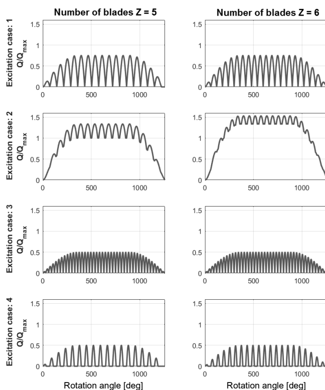
Figure 5 : Propeller ice torque excitation for 5 and 6 blades
