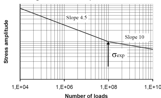
Figure 8 : Constant-slope S-N curve
