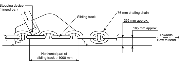
Bar hinged type chain stopper
