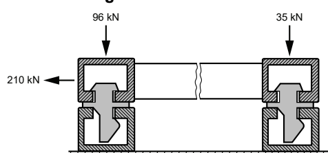
Figure 7 : Shear test
