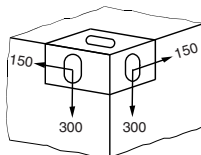
Figure 19 : Resultant permissible load on container corners
