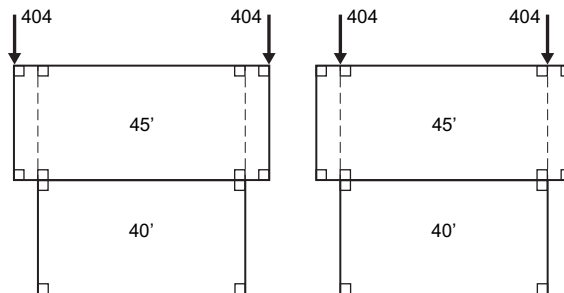
Figure 15 : Permissible vertical compression on frames of 45' ISO containers topped on 40' containers
