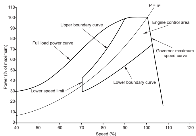
Figure 2 : Control area for variable speed propulsion engine
