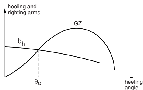
Figure 1 : Heeling and righting arm curves
