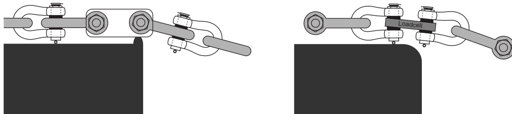
Figure 8 : Schematic of calibration procedure according to ISO 7500-1:2018
