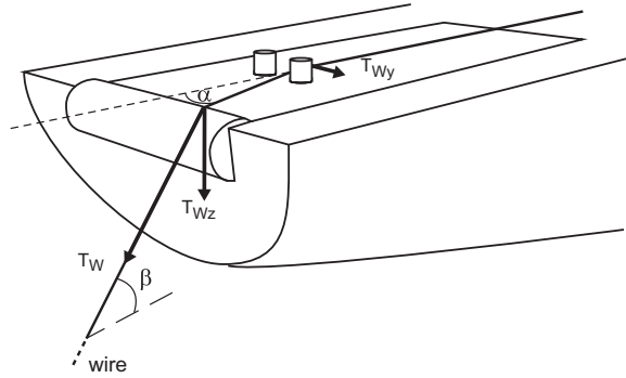
Figure 2 : Tension and position of wire
