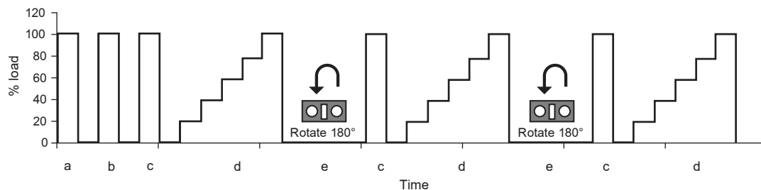
Figure 8 : Schematic of calibration procedure according to ISO 7500-1:2018
