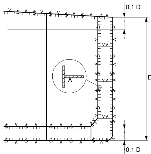
Figure 15 : Location of measurements on transverse section of CSR oil tankers
