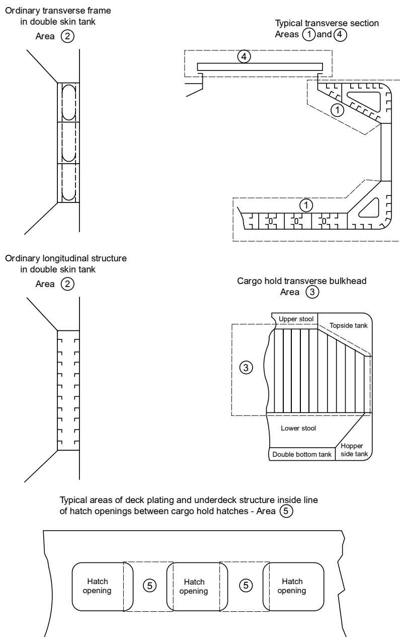
Figure 4 : Areas subject to close-up surveys and thickness measurements for double skin bulk carriers
