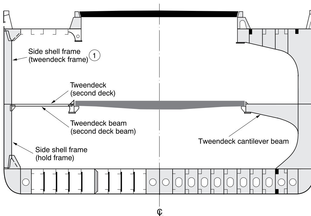
Figure 4 : Areas subject to close-up surveys and thickness measurements of general cargo ships
