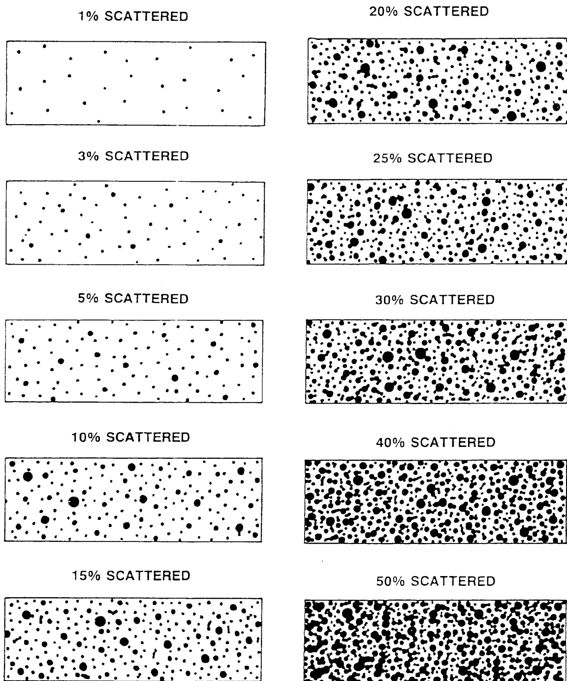
Figure 22 : Pitting intensity diagrams (from 1% to 50% intensity)
