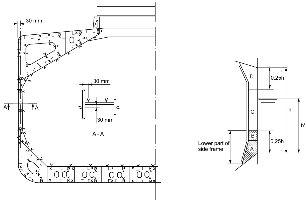
Figure 11 : Location of measurements on structural members in cargo holds and ballast tanks of CSR single skin bulk carriers
