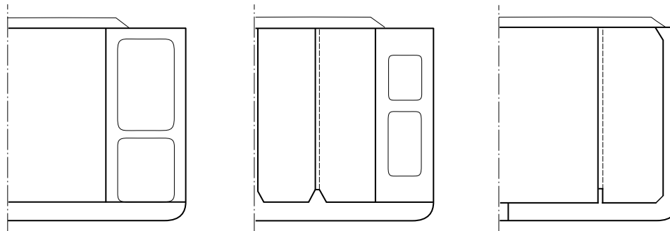
Figure 8 : Typical midship sections of ships with service notation chemical tanker ESP
