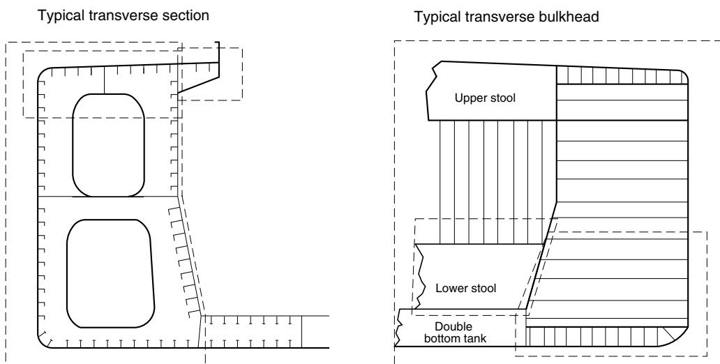
Figure 4 : Areas subject to close-up surveys and thickness measurements for double skin bulk carriers
