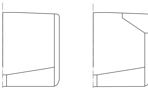
Figure 6 : Typical midship sections of ships with service notation cement carrier
