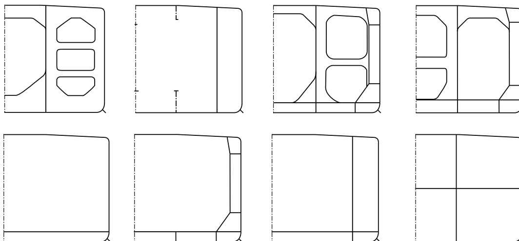
Figure 7 : Typical midship sections of ships with service notation oil tanker ESP
