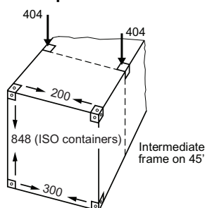
Figure 13 : Permissible transverse and vertical compressions on end and intermediate frames of 45' ISO containers
