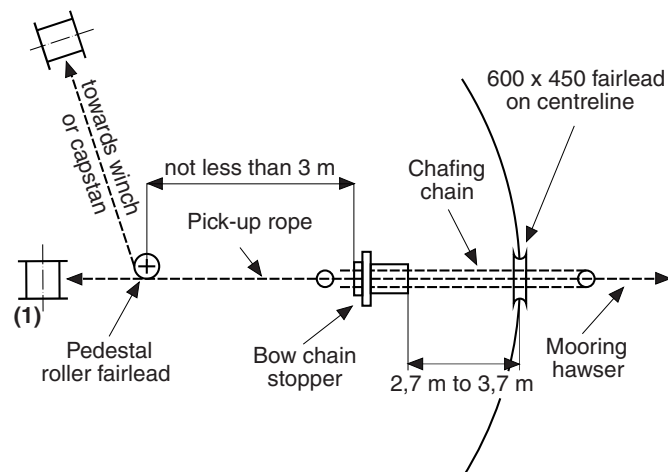
Figure 2 : Forecastle schematic layout for DWT ≤ 150000 t
