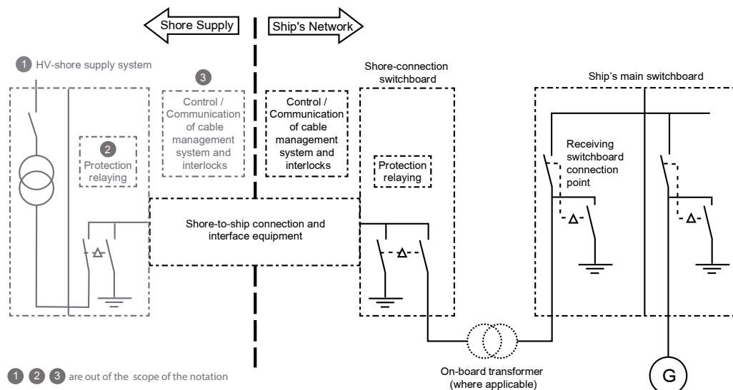
Figure 1 : Diagram of a typical OPS arrangement
