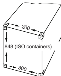
Figure 12 : Permissible transverse and vertical compressions on end frames of 20', 30' and 40' ISO containers
