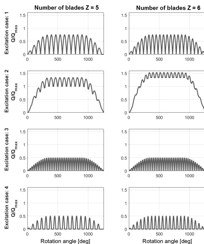
Figure 5 : Propeller ice torque excitation for 5 and 6 blades
