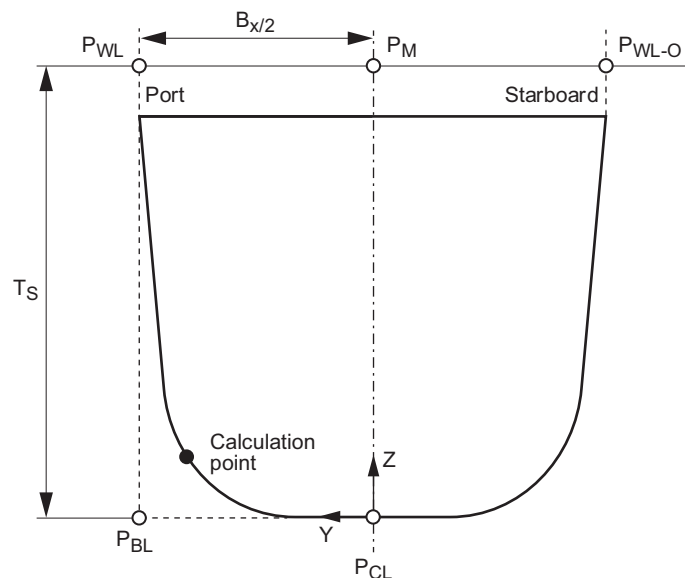
Figure 1 : Hydrodynamic pressures in temporarily submerged condition
