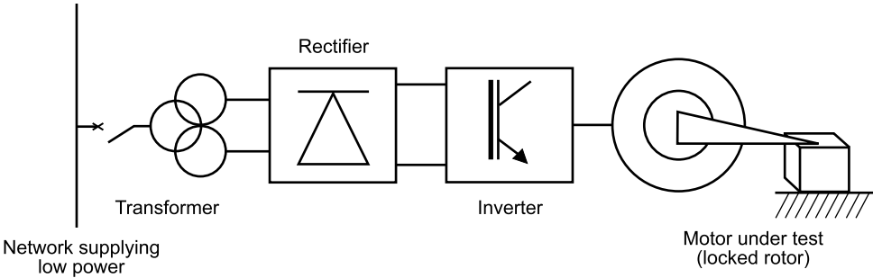
Figure 1 : Heating Test 1
