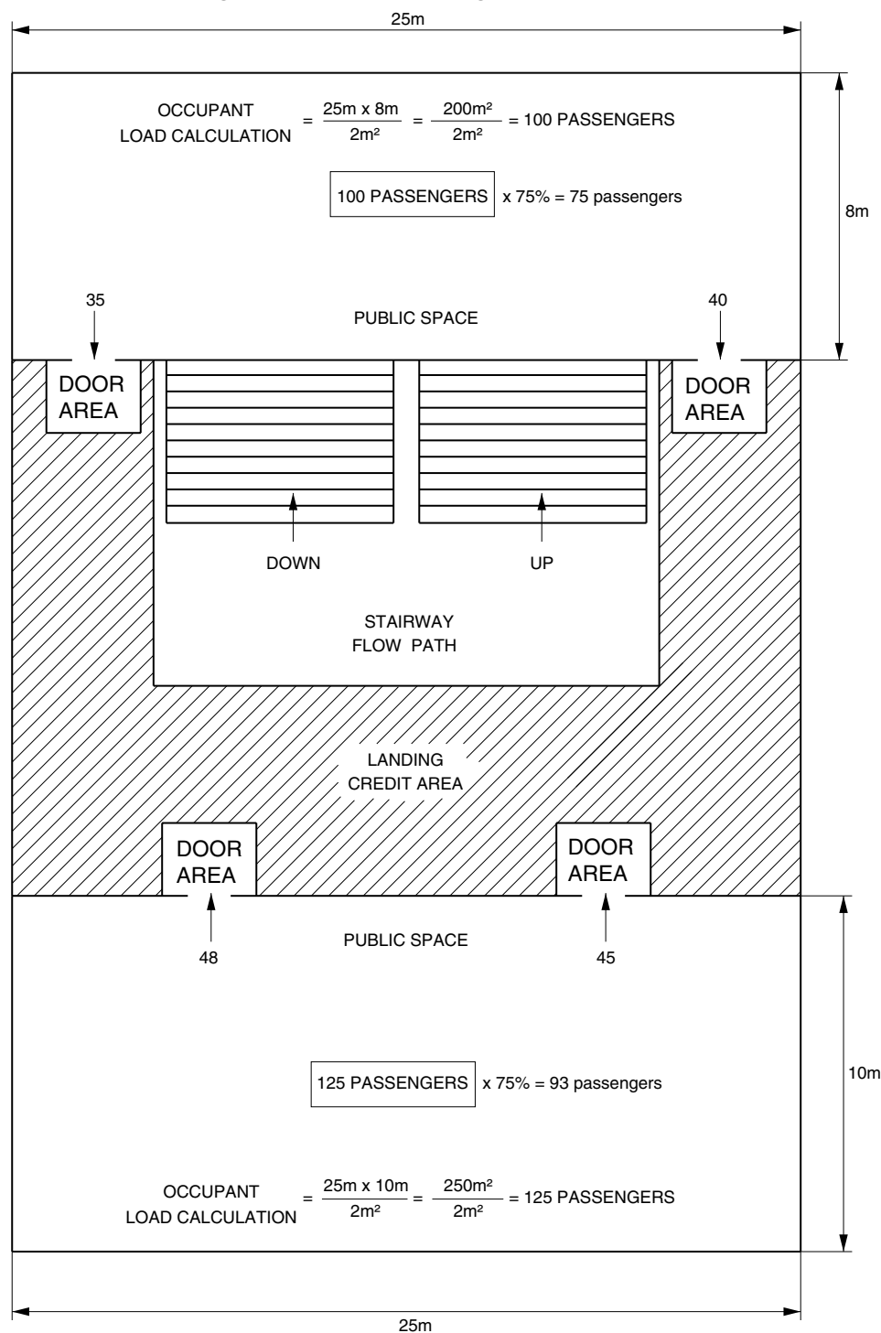
Figure 3 : Occupant loading calculation example
