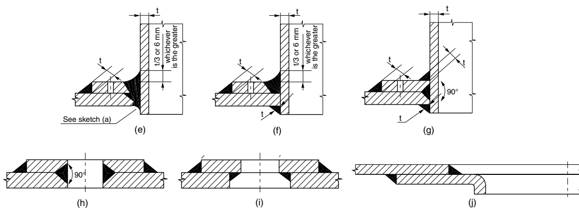
Figure 31 : Types of joints for nozzles and reinforcing rings (2)
