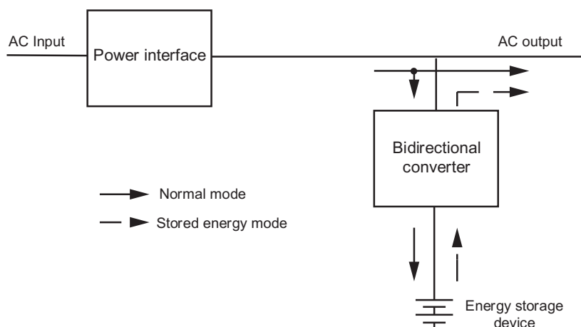
Figure 2 : Line-interactive topology
