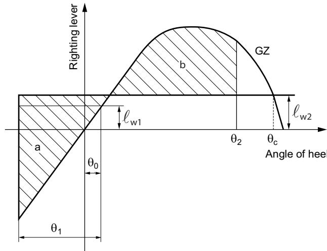
Figure 2 : Righting lever curve for wind propulsion system in stand-by mode for ship more than 500GT
