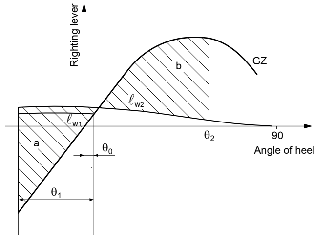
Figure 1 : Righting lever curve for wind propulsion system in stand-by mode for ship less than 500GT
