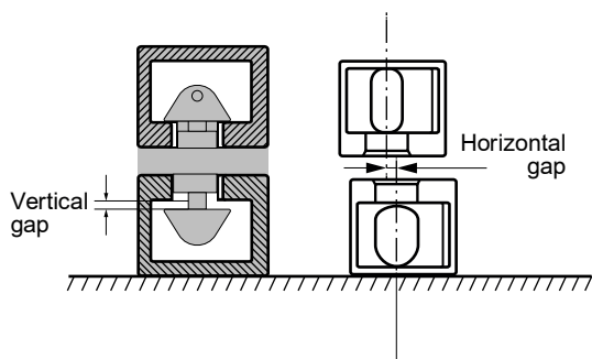
Figure 2 : Horizontal and vertical gaps
