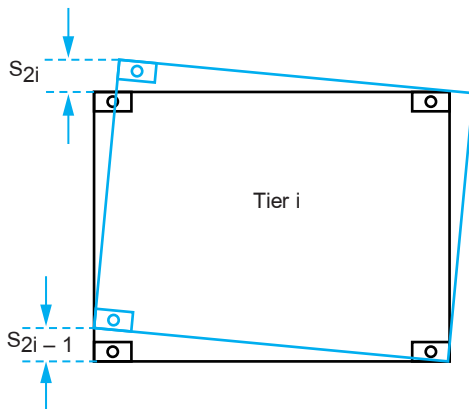
Figure 8 : Vertical displacements (positive)
