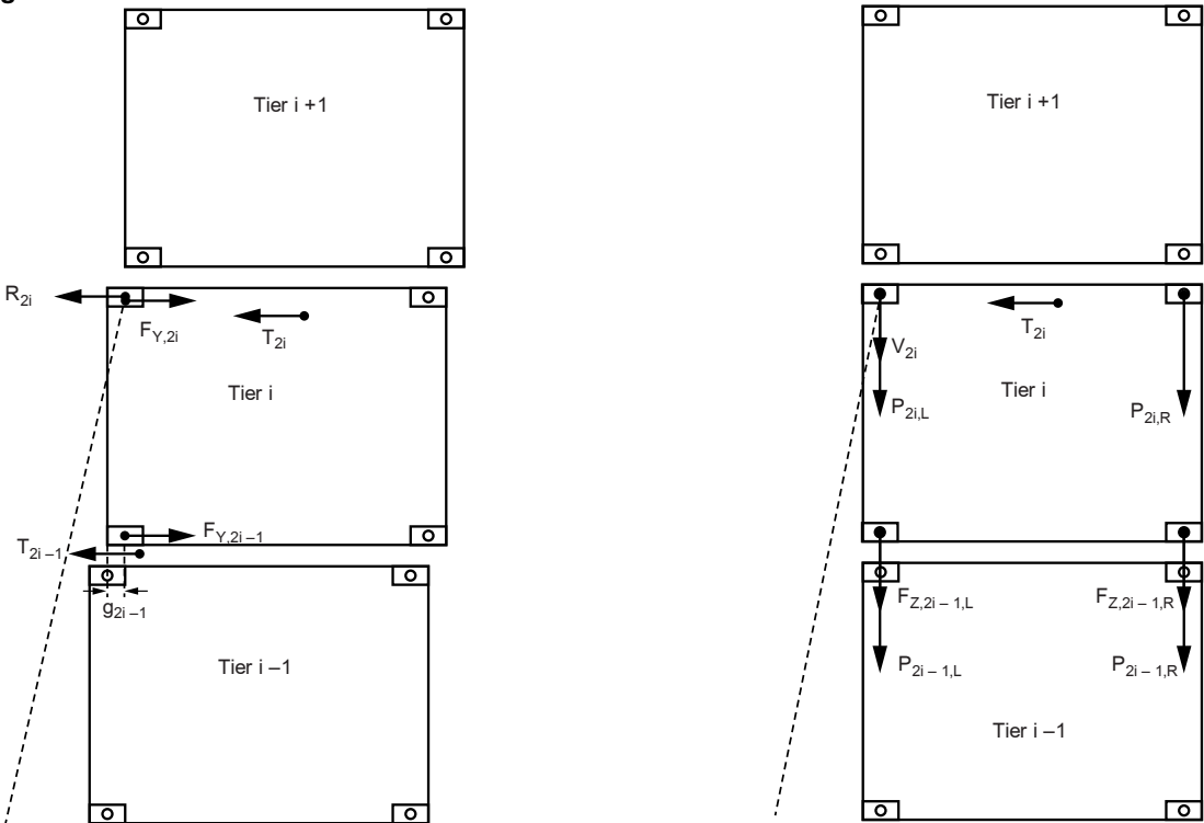
Figure 6 : Vertical lashing reactions and forces
