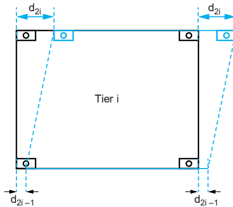
Figure 5 : Horizontal displacements (negative)
